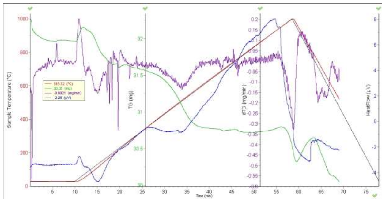
Figure 3. Activated bentonite derivativeogram
