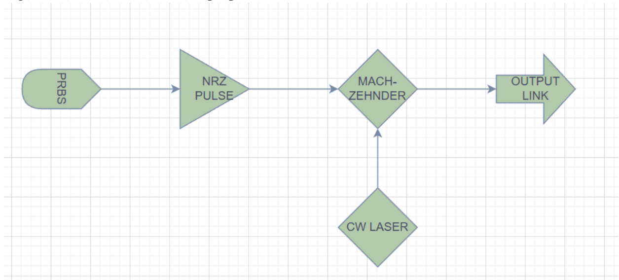
Fig 6 transmitter circuit
