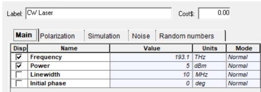
Fig.3 (CW)laser properties
